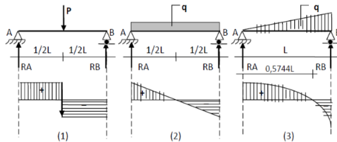
Gambar 2.19 Diagram Gaya Lintang
